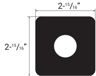
SQUARE ROSE DIMENSIONS
